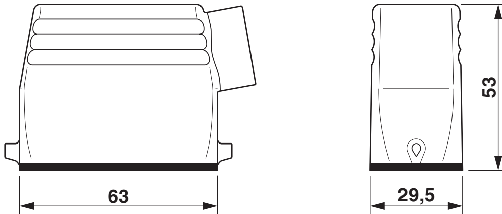
Dimensional drawing
